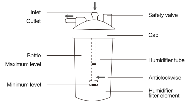
Figure 4: Humidifier Components
