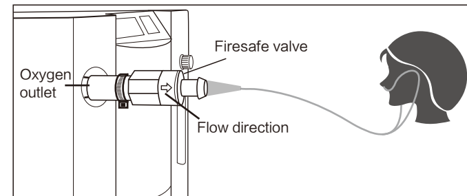
Figure 7: Firesafe valve
